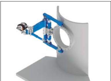
BASE CLAMP-ON
